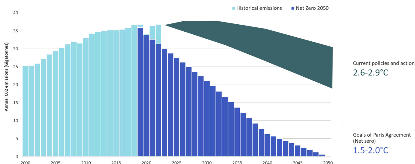
Figure 1: 2100 warming projections
